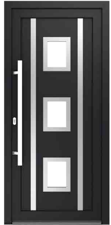
OHIO INOX
